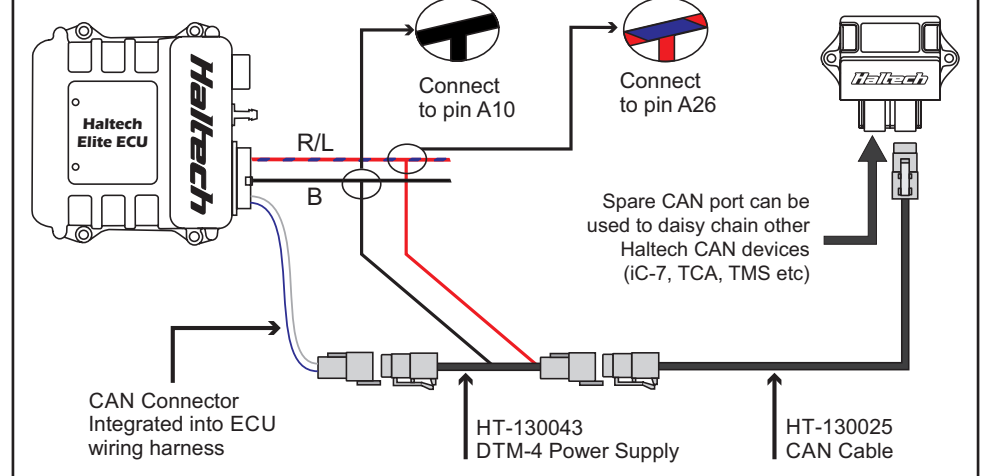
Haltech WB1 connected to Elite series single connector ECU
