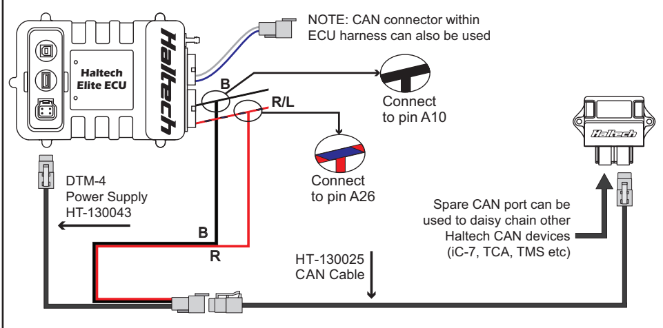
Haltech WB1 connected to Elite series dual connector ECU
